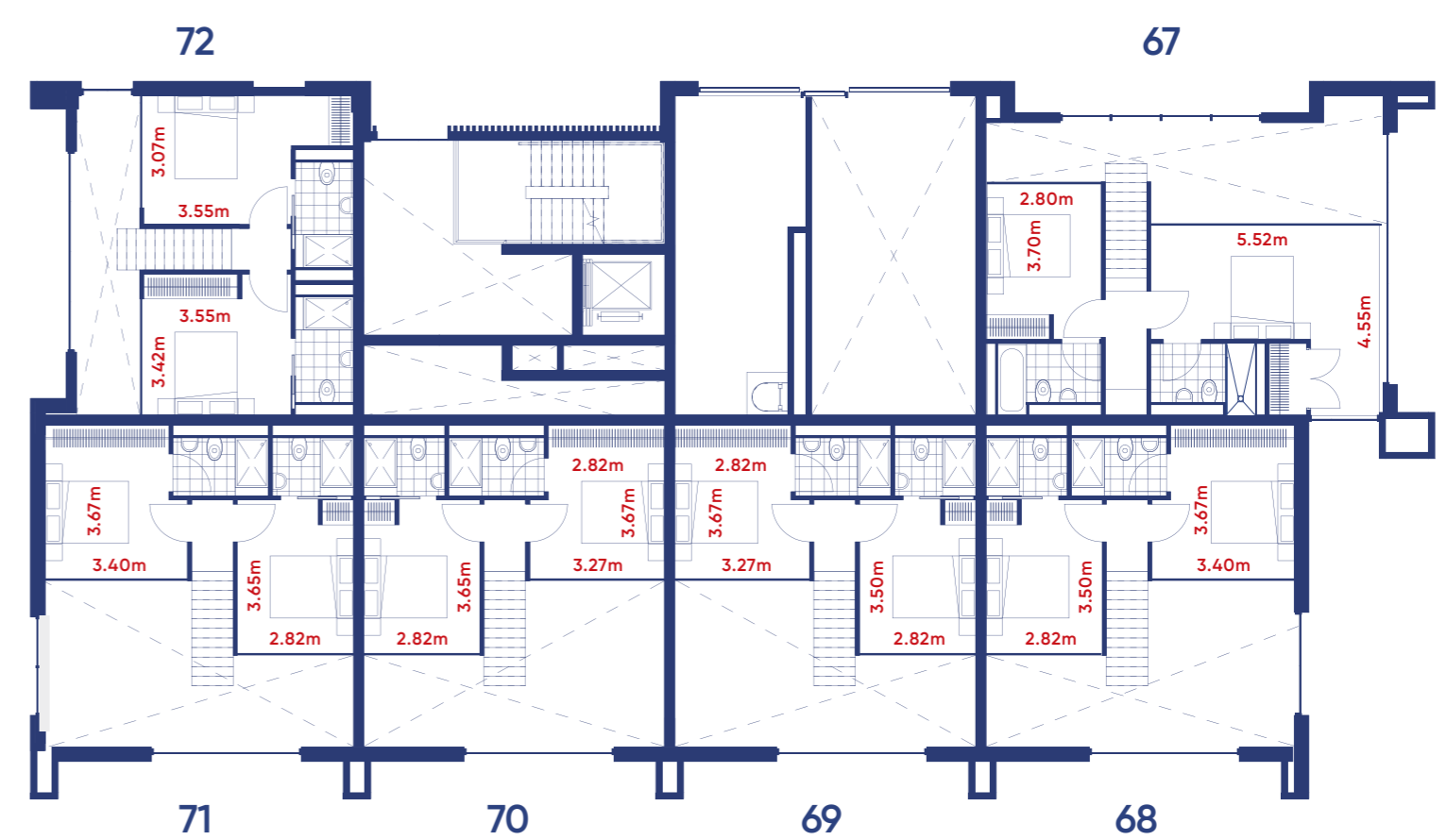
Mezzanine plan
